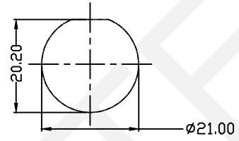
PANEL CUT-OUT Thickness 3.0mm Max
