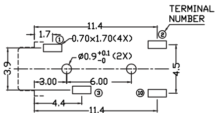
PCB LAYDUT <BOTTOM VIEW>
