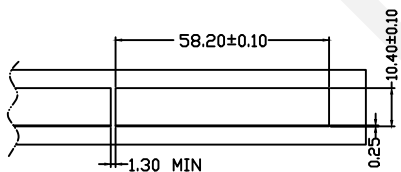
RECOMMENDED BEZEL CUT-OUT
