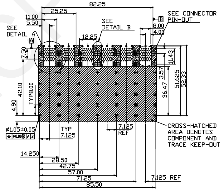
RECOMMENDED PC BOARD LAYOUT AS VIEWED FROM COMPONENT SIDE TOLERANCE ±0.05mm
