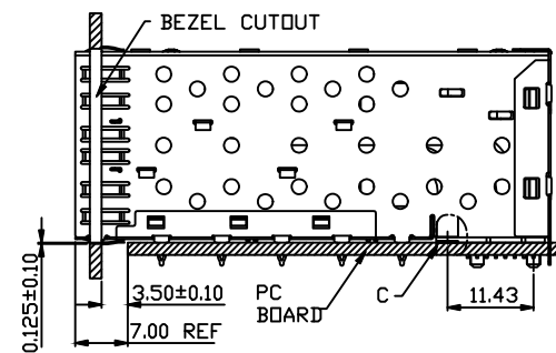
BEZEL CUT-OUT CENTER SPACING DETAIL BEZEL THICKNESS:0.8-2.6
