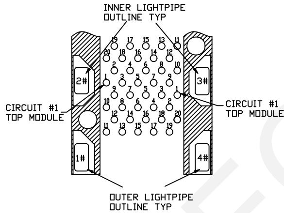
CONNECTOR PIN-OUT COMPONENT SIDE OF BOARD
