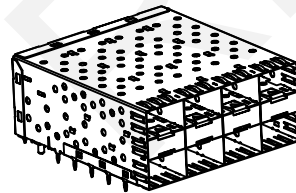
RHTLYFP-024 WITHOUT LIGHT PIPES
