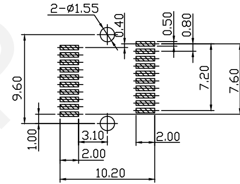
Detail A (2:1)
