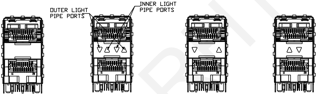
RHTLYFP-013 2x1 Press Fit WITHOUT LIGHT PIPES
