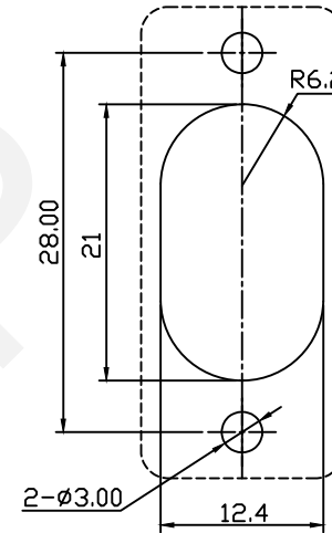
PANEL CUT-OUT
