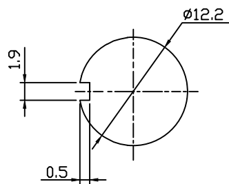
Panel Mounting
