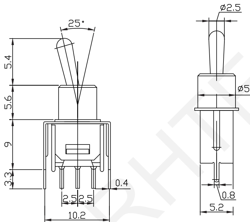
Outline Drawing
