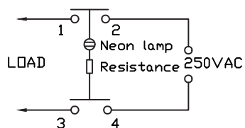
Circuit of switch
