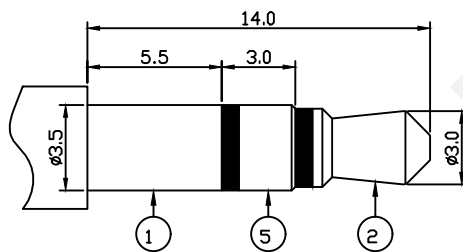
Ø3.50mm 3 POLE PLUG
