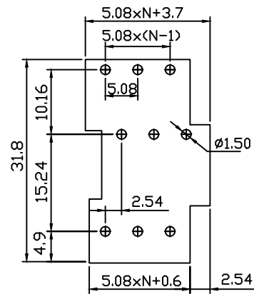
PCB LAYOUT
