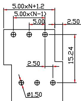
PCB LAYOUT
