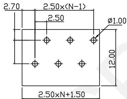
B type PCB LAYOUT
