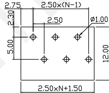
A type PCB LAYOUT
