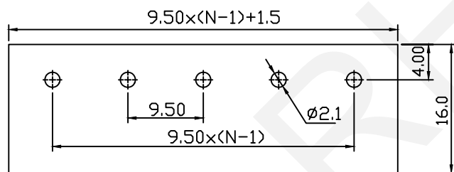
PCB LAYOUT
