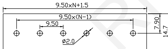
PCB LAYOUT
