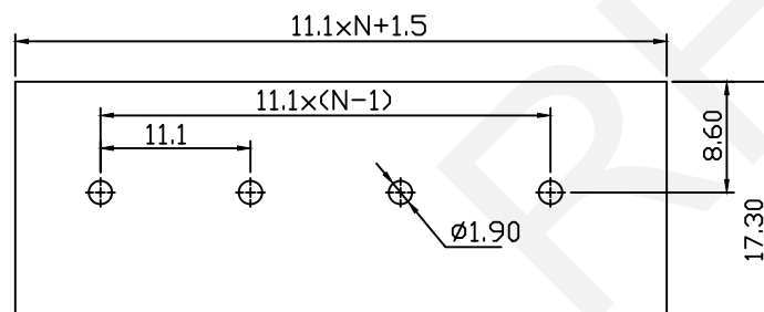
PCB LAYOUT
