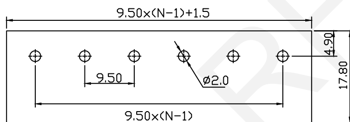
PCB LAYOUT
