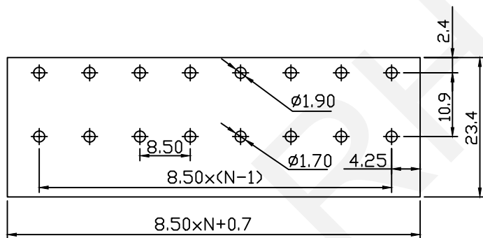
PCB LAYOUT
