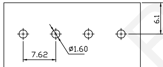
PCB LAYOUT
