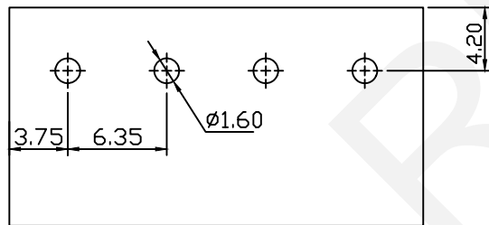
PCB LAYOUT
