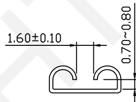
SECTION A-A (2:1)
