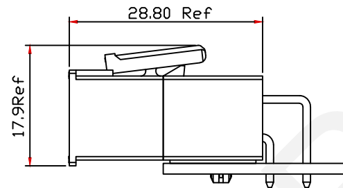
MATED DRAWING
