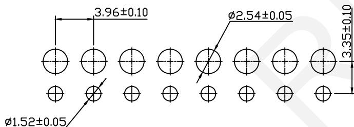
PCB LAYOUT
