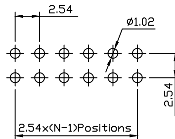
Recommended P.CB Layout(Top Side) (PCB BOARD TOLERANCE±0.05)
