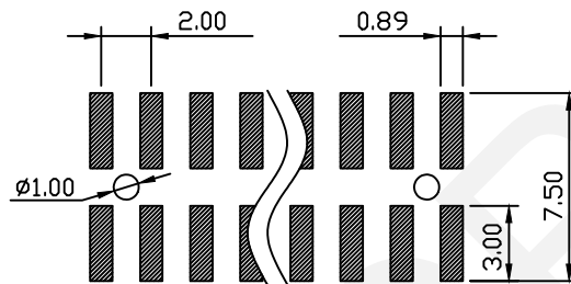
Recommended P.CB Layout (Top Side) (PCB BOARD TOLERANCE \pm 0.05 )
