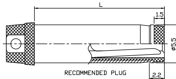
SCHEMATIC
