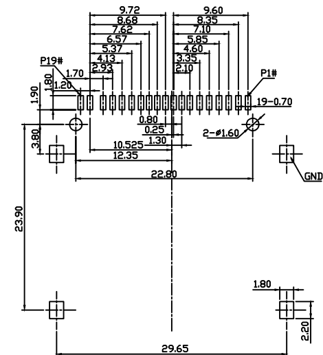
RECOMMENDED PCB LAYOUT TOLERANCE UNLESS OTHERWISE IS±0.05
