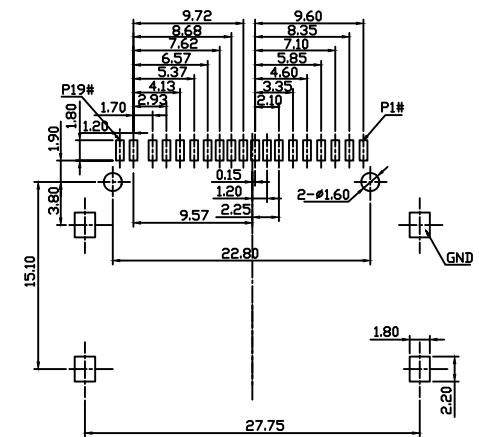
RECOMMENDED PCB LAYOUT TOLERANCE UNLESS OTHERWISE IS±0.05
