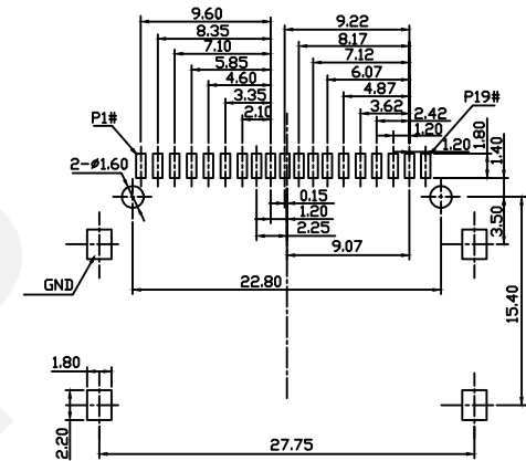
RECOMMENDED PCB LAYOUT TOLERANCE UNLESS OTHERWISE IS±0.05
