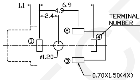
PCB LAYOUT (BOTTOM MEW)
