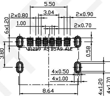
RECOMMENDED PCB LAYOUT GENERAL TOLERANCE: ±0.05mm
