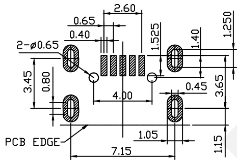
RECOMMENDED PCB LAYOUT TOL±0.05
