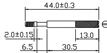
Long Screw
