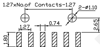
Recommended P.C.B Layout(Top Side) (PCB BOARD TOLERANCE±0.05)
