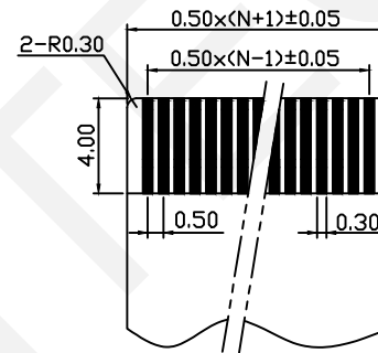
Proper Cable
