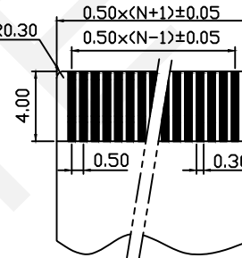
Proper Cable
