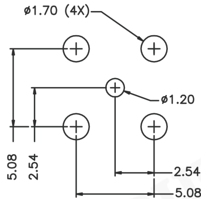
PCB MOUNTING HOLES
